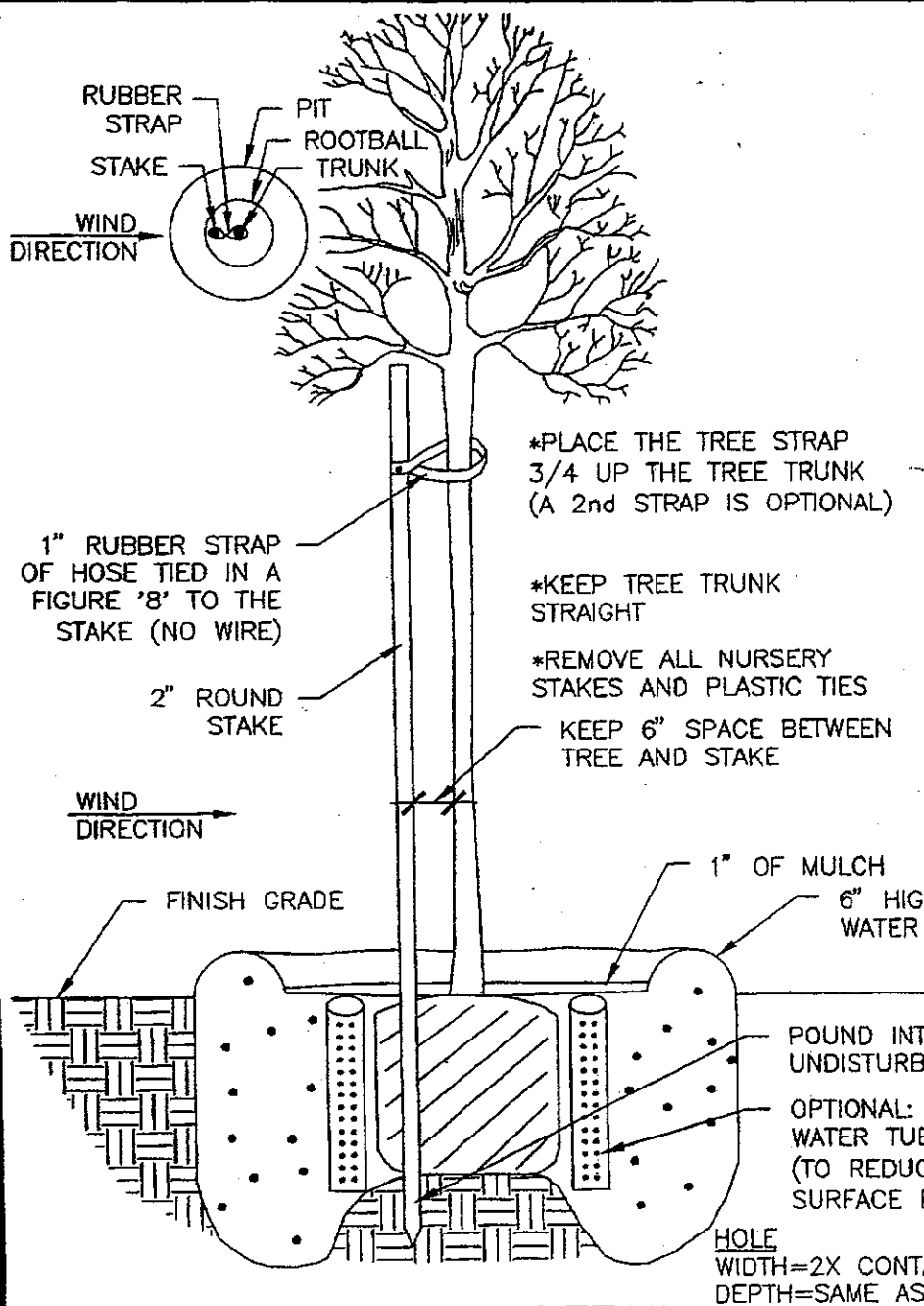
PLANTING DETAIL FOR A 15 GALLON SIZE TREE
