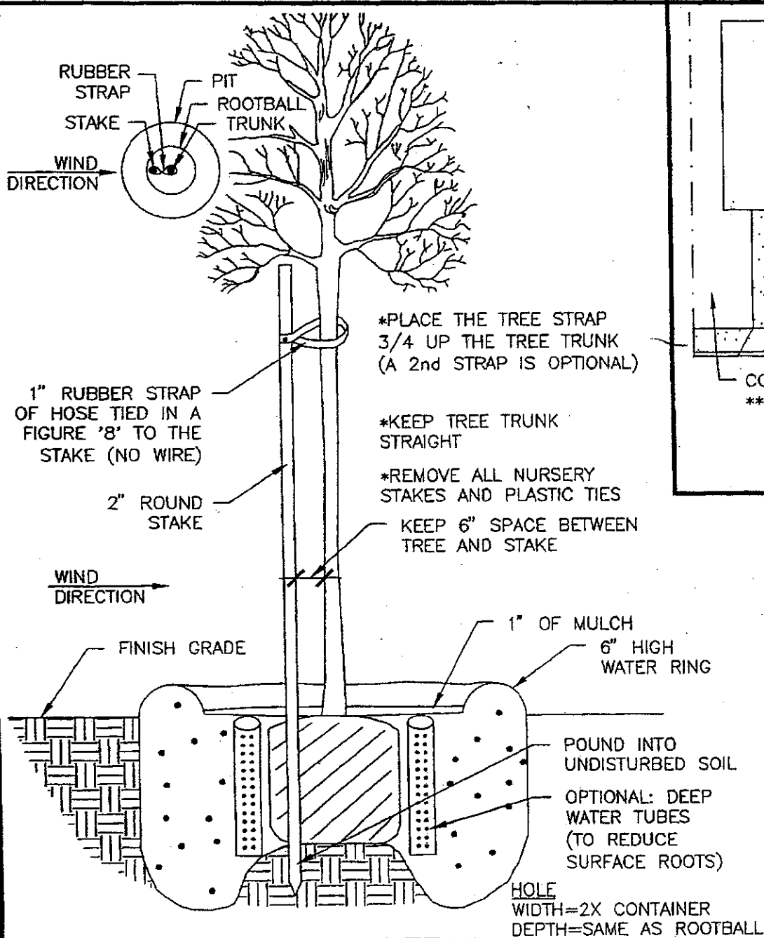
PLANTING DETAIL FOR A 15 GALLON SIZE TREE
